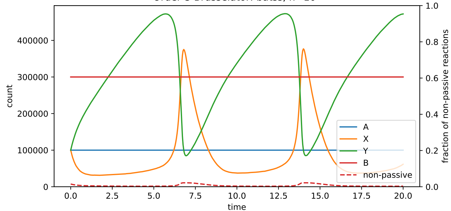
Order-3 Brusselator: batss, n=10^5
